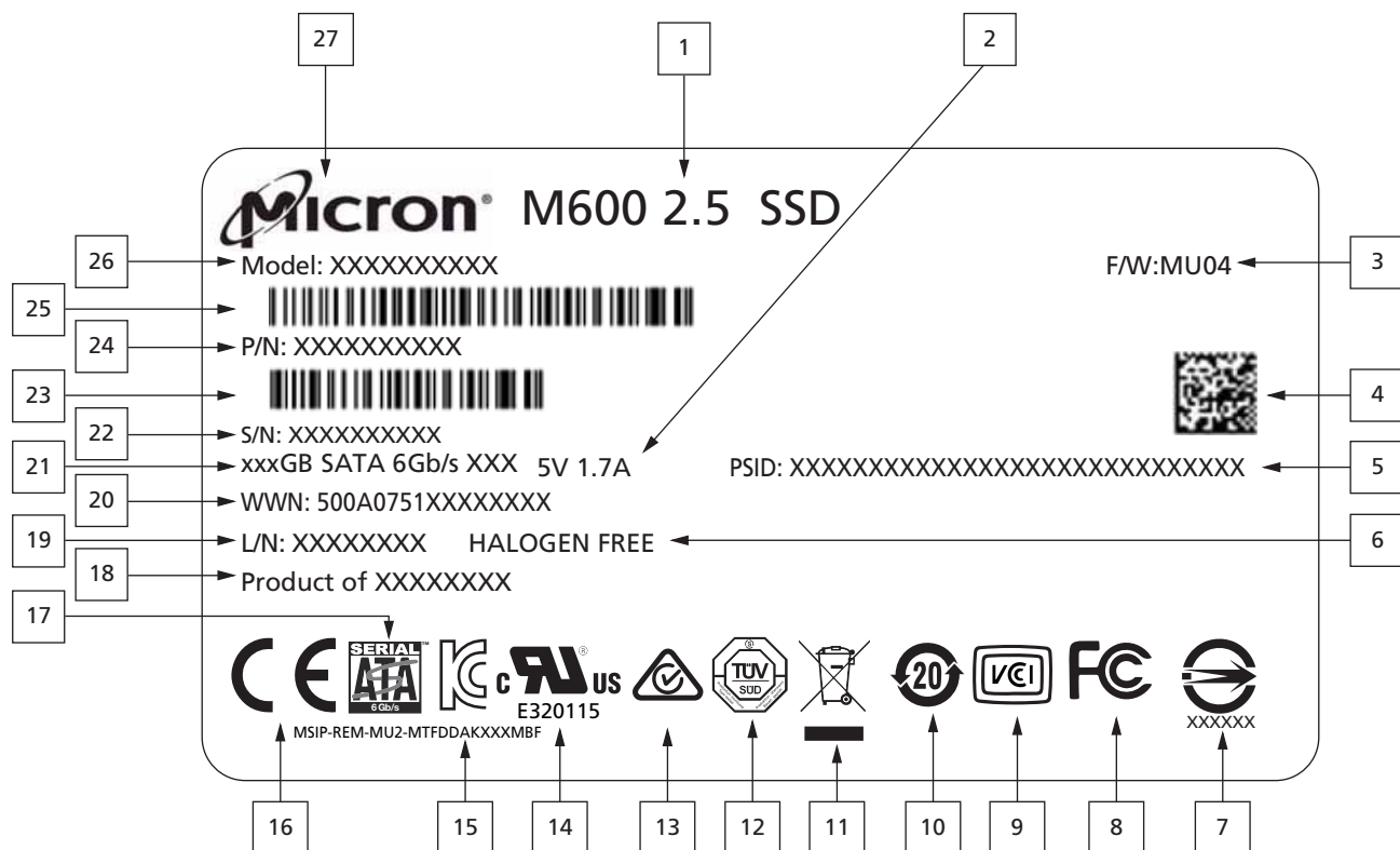
Figure 9: 2.5-inch Label Structure – M5XX(DC/IT)/M600
