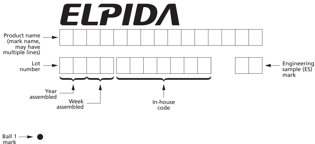
Figure 3: Legacy BGA Component with Elpida Part Mark
