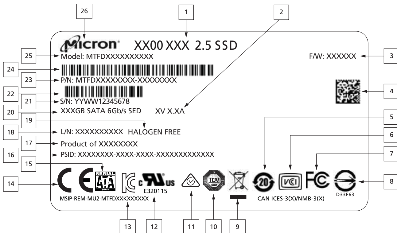
Figure 8: Micron Standard 2.5 SSD Label Structure
