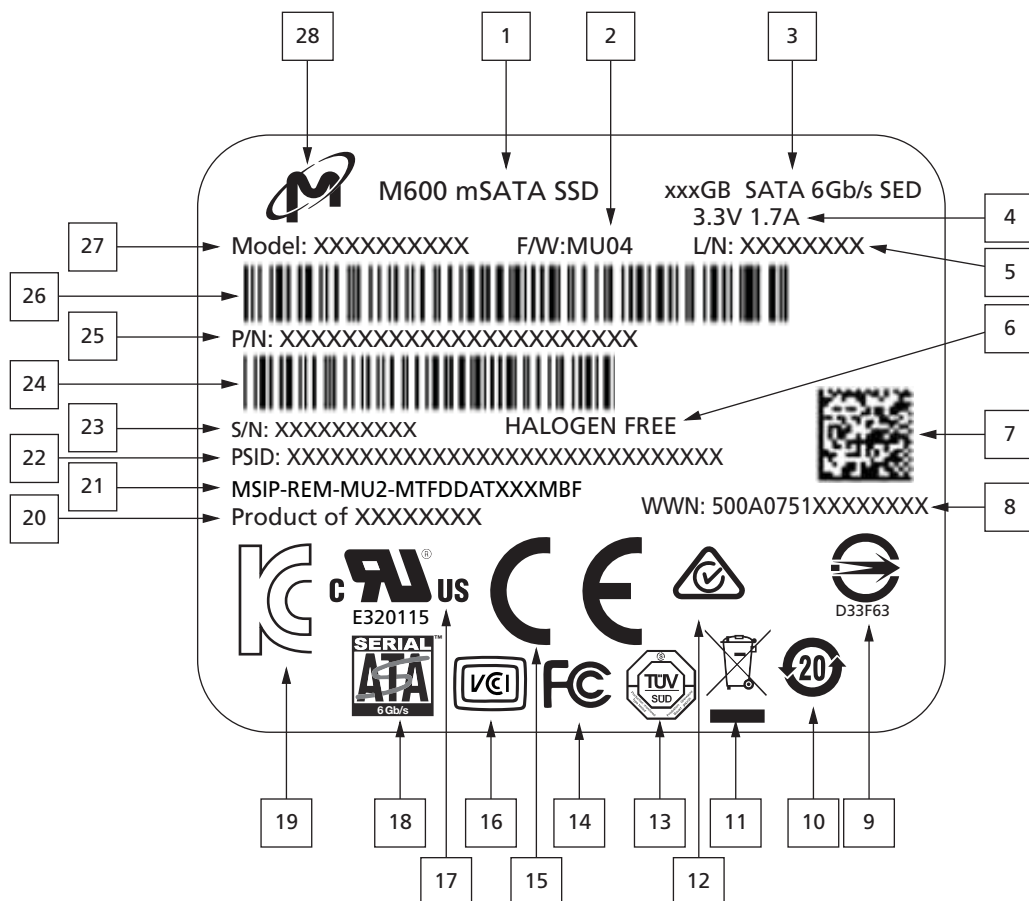
Figure 11: mSATA Label Structure – M6XX
