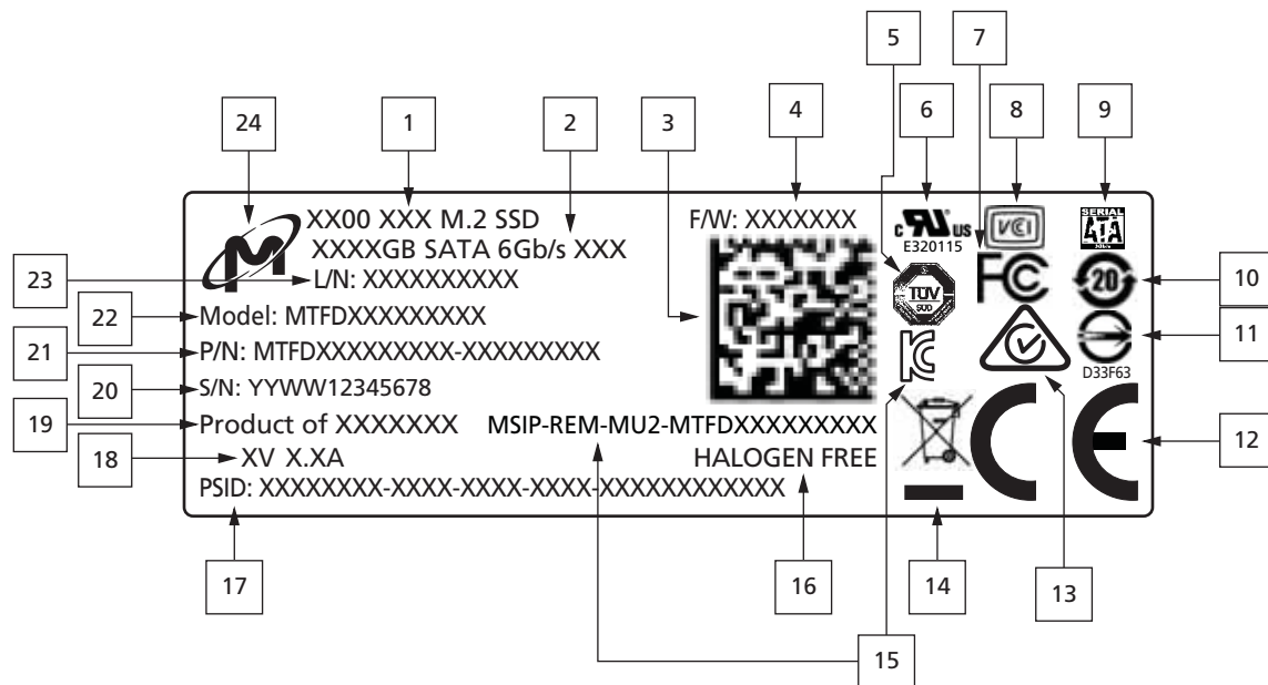
Figure 10: Micron Standard M.2 SSD Label Structure
