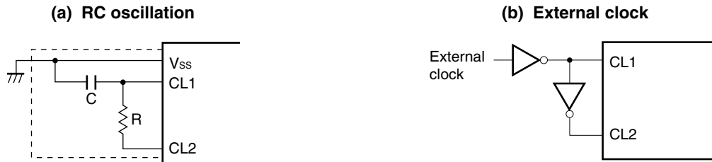
Figure 5-10. External Circuit of External RC Oscillator
