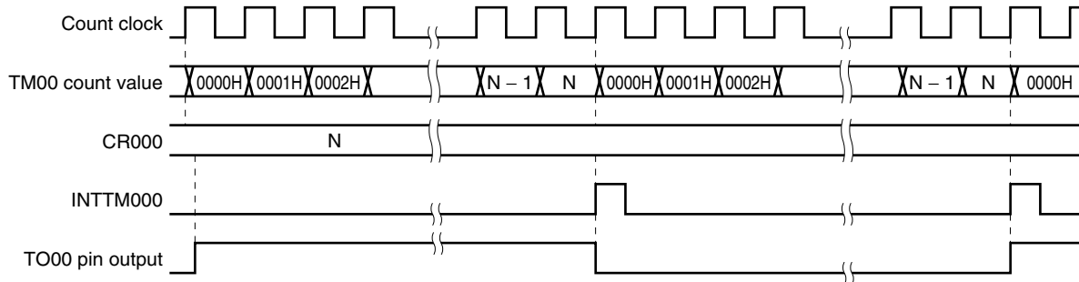
Figure 6-30. Square-Wave Output Operation Timing
